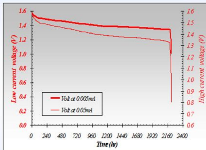
Battery model : PBP5555, @21°C
